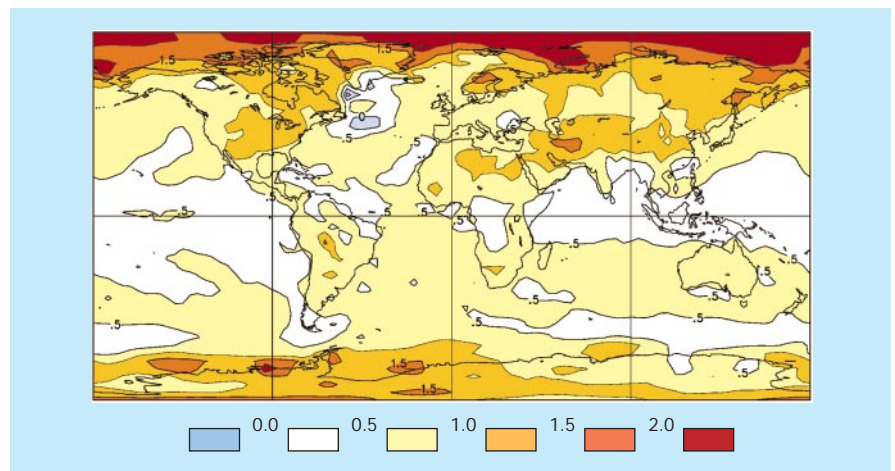
Figure 1 A warmer world. Shown here are projected changes in surface air temperature, relative to 1990–2000, for the decade 2020–30. The global change in mean temperature estimated by this model 15 , the Canadian Centre for Climate Modelling and Analysis CGCM2, is 0.68 K. This result is similar to that obtained by other atmosphere–ocean global climate models, such as that used by Stott and Kettleborough 4 . It is also similar to the conclusions drawn by Knutti et al. 3 from a model of intermediate complexity. The change projected by CGCM2 falls well within the approximate 5–95% uncertainty ranges estimated by Stott and Kettleborough (0.3–1.3 K) and by Knutti et al. (0.5–1.1 K). The global change in mean temperature is expected to have an uneven distribution geographically, with generally greater warming over land and at high latitudes than elsewhere. So local effects of climate change may be greater than one might infer from global mean projections.
