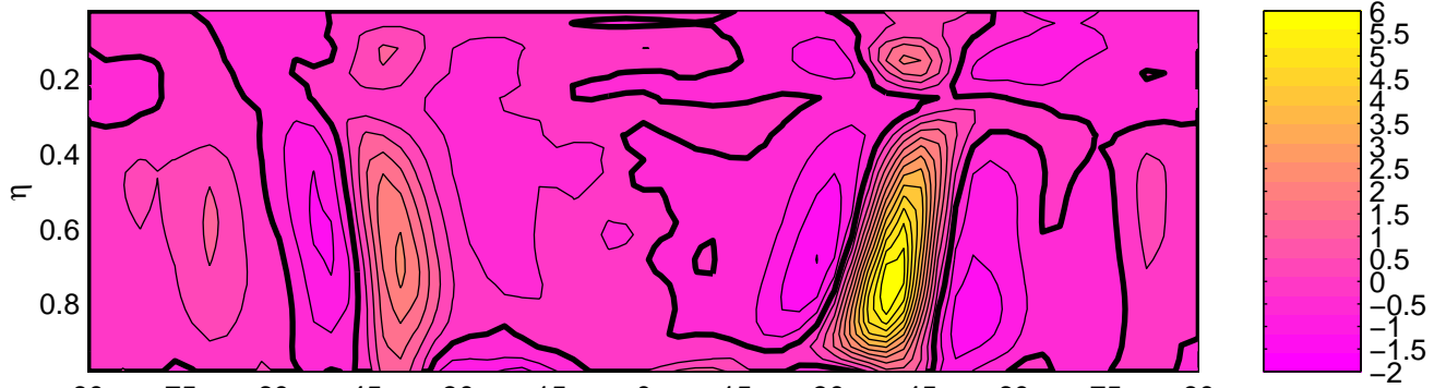
\langle |U_m|^2 \rangle_{\eta t} by 0.25 (m 2 s -2 )
