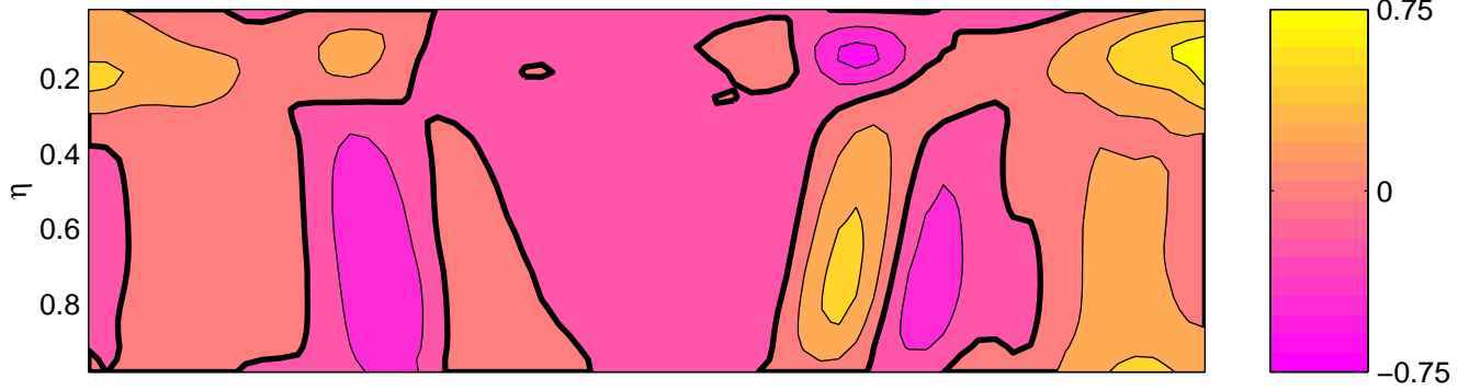
\langle T^2 \rangle_{\lambda t} by 0.5 (K 2 )
