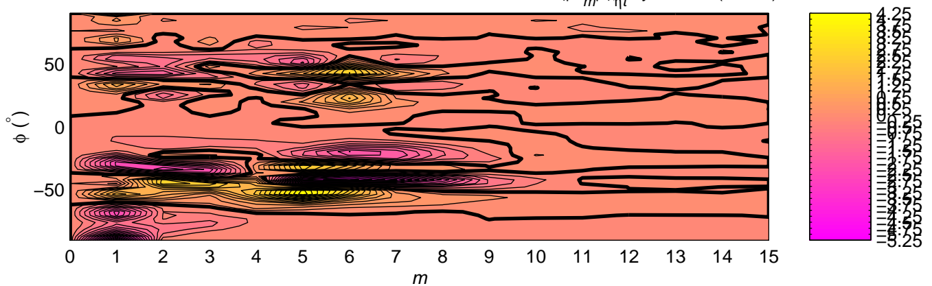
\langle U_m^2 \rangle_{\eta t} by 0.25 \text{ (m}^2\text{s}^{-2}\text{)}
