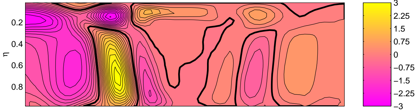
\langle T^2 \rangle_{\lambda t} by 0.5 \text{ (K}^2\text{)}
