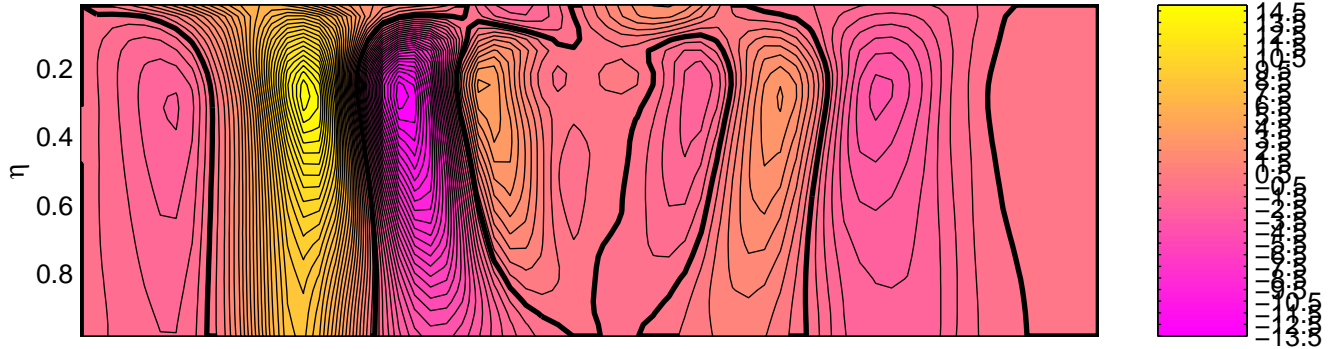
\langle T \rangle_{\lambda t} by 0.25 \text{ (K)}
