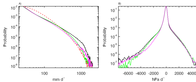
Figure 3. (a) PDFs of precipitation rates for August 2005 between 30°S and 30°N for experiments defined in Table 2: CTR (black curve); CL1 (green curve); and CL2 (magenta curve). The corresponding TRMM 3B42 observational estimate is shown by the dashed red curve. Note results are displayed in log-log form. (b) Same as except for vertical motion around 850 hPa ( \omega_{850} ) over ocean, between 12°S and 25°S. Note only vertical axis is logarithmic in Figure 3b. Probabilities are with respect to bins of 15 mm d -1 (Figure 3a) and 80 hPa d -1 (Figure 3b).
