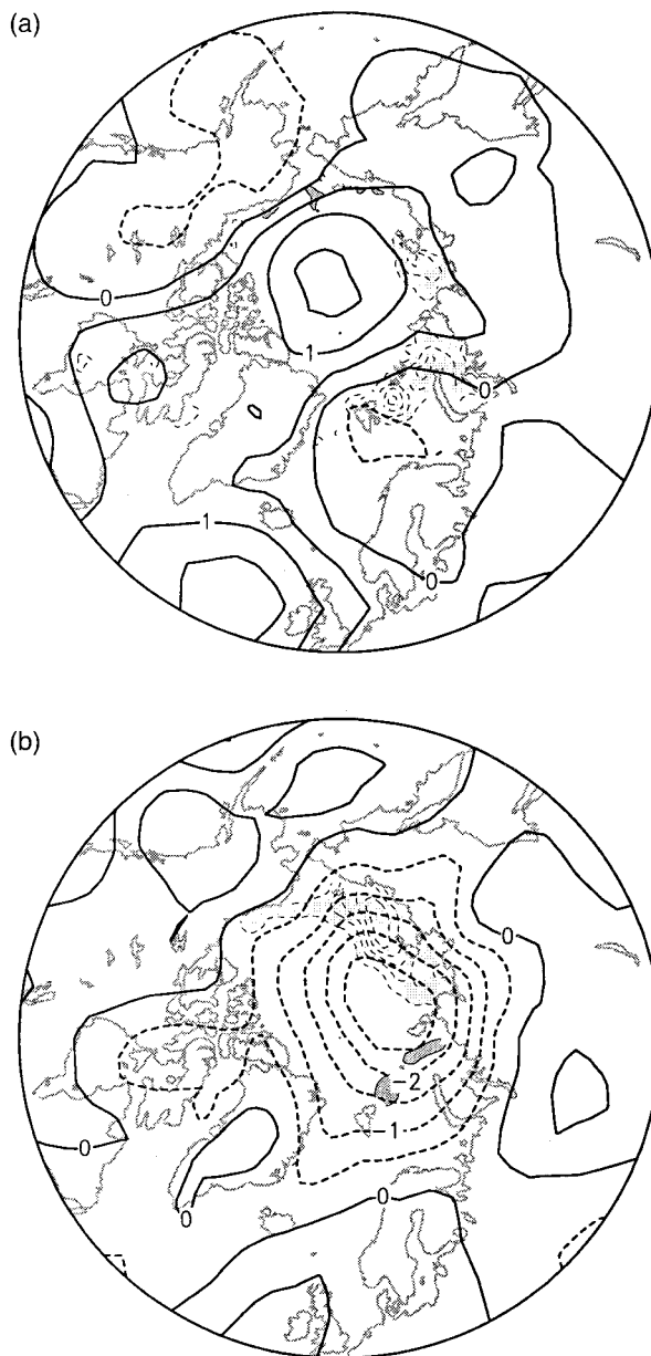
FIG. 17. (a) Regression map of spring (April-June) SLP (thick contours) and summer (July-September) sea ice concentration (shading and thin contours) anomalies based upon the record of summer ice extent in the region ( 20^{\circ} - 135^{\circ} E) during the period 1958-78. Both the SLP and ice regression fields have been multiplied by -1 . Units are mb for SLP (ice concentration). Light (dark) shading denotes ice concentration values less than -5\% (greater than 5\% ) per unit standard deviation of the ice extent index. The contour interval is 5\% per decade, and the zero contour has been omitted. (b) As in (a), but based on summer ice extent in the region ( 135^{\circ} E- 180^{\circ} ) during the period 1979-96.
